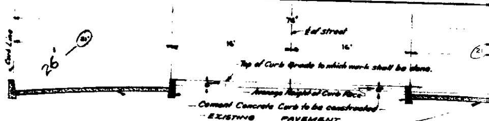
TYPICAL SECTION OF STREET (27TH ST. TO MARSHALL) SCALE (HORIZONTAL) 1"=20' (VERTICAL) 1"=4'
